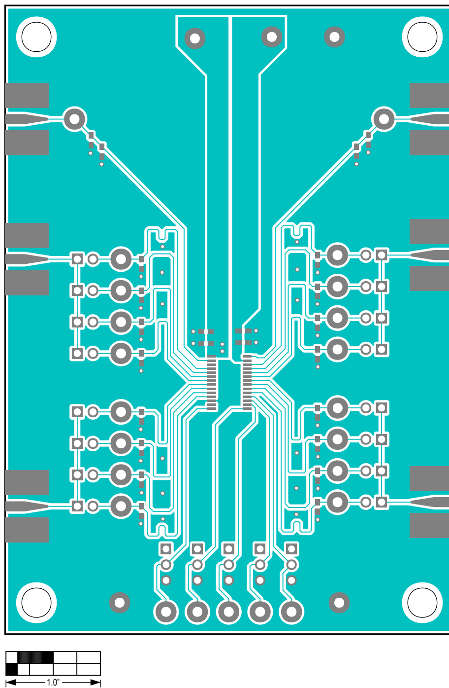
DG1206-1207 EV Kit PCB Layout — Top View
