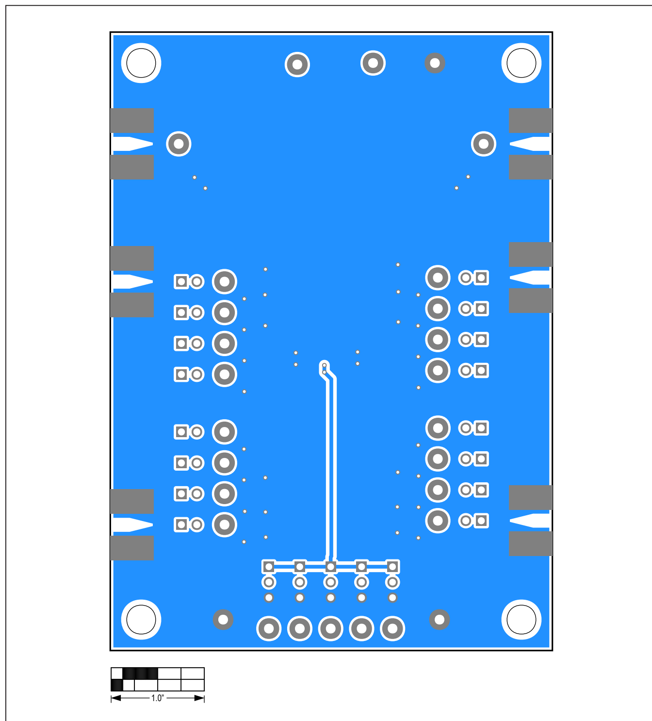
DG1206-1207 EV Kit PCB Layout — Bottom View
